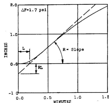
FIG. 8 REACTION CURVE
